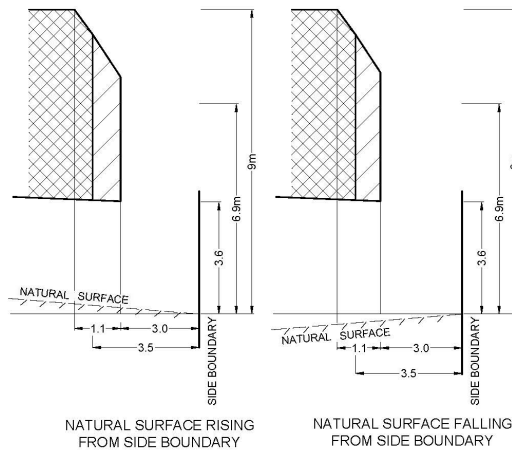
(C) PROFILE
