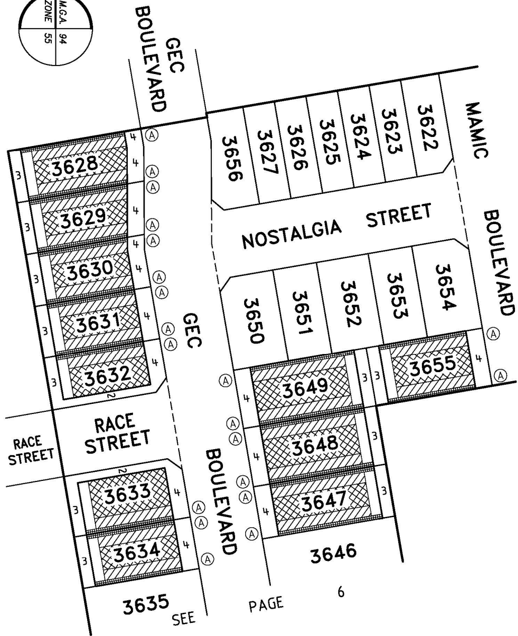
BUILDING ENVELOPE DIAGRAM
