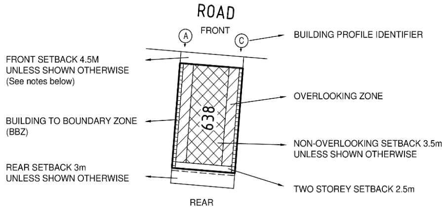
EXAMPLE OF TYPICAL BUILDING ENVELOPE SETBACKS
