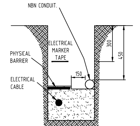
TYPICAL SECTION TRENCH ARRANGEMENT - LV NOT TO SCALE
