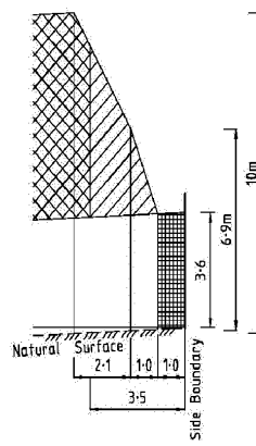
Natural surface falling from side boundary
