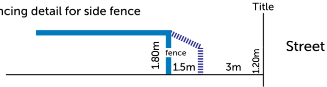
2. Fencing template for standard lot
