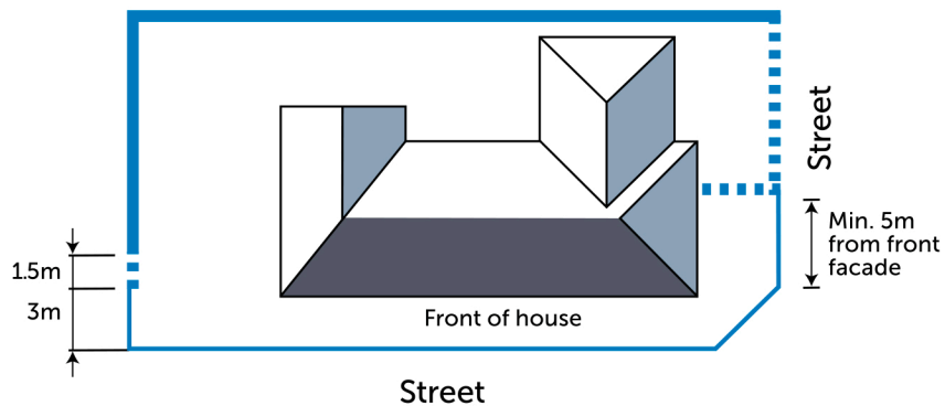
4. Fencing template for corner lot (b)
