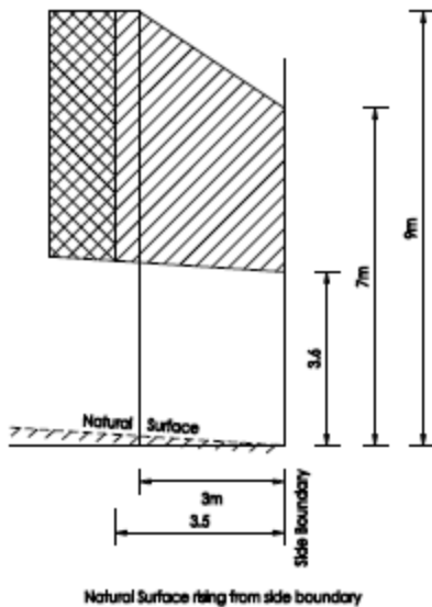
T Profile - SIDE BOUNDARY
