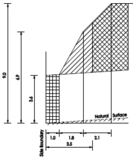
B Profile - SOUTH Boundary
