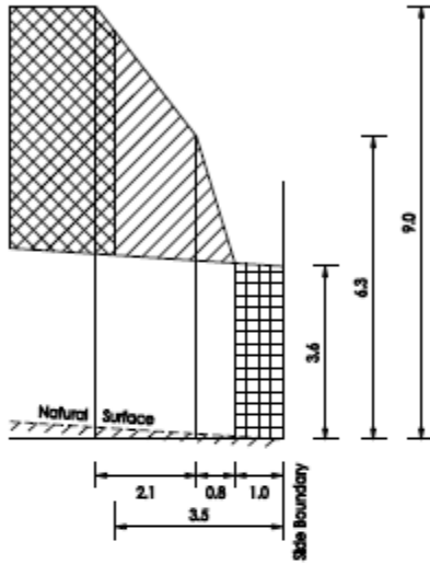
A Profile - NORTH, EAST or WEST Boundary
