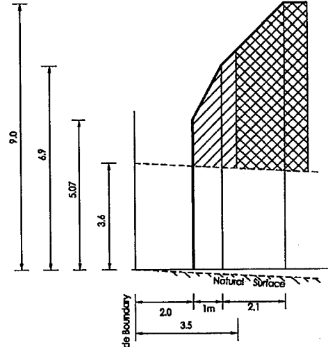
Natural Surface falling from side boundary
