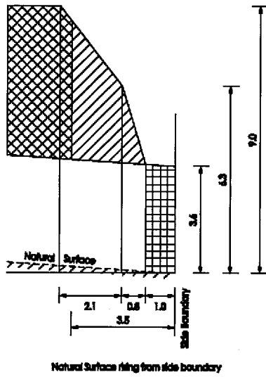
(A) Profile - NORTH, EAST or WEST boundary
