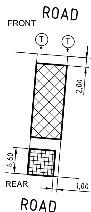
EXAMPLE OF REAR LOADED TERRACE LOT
