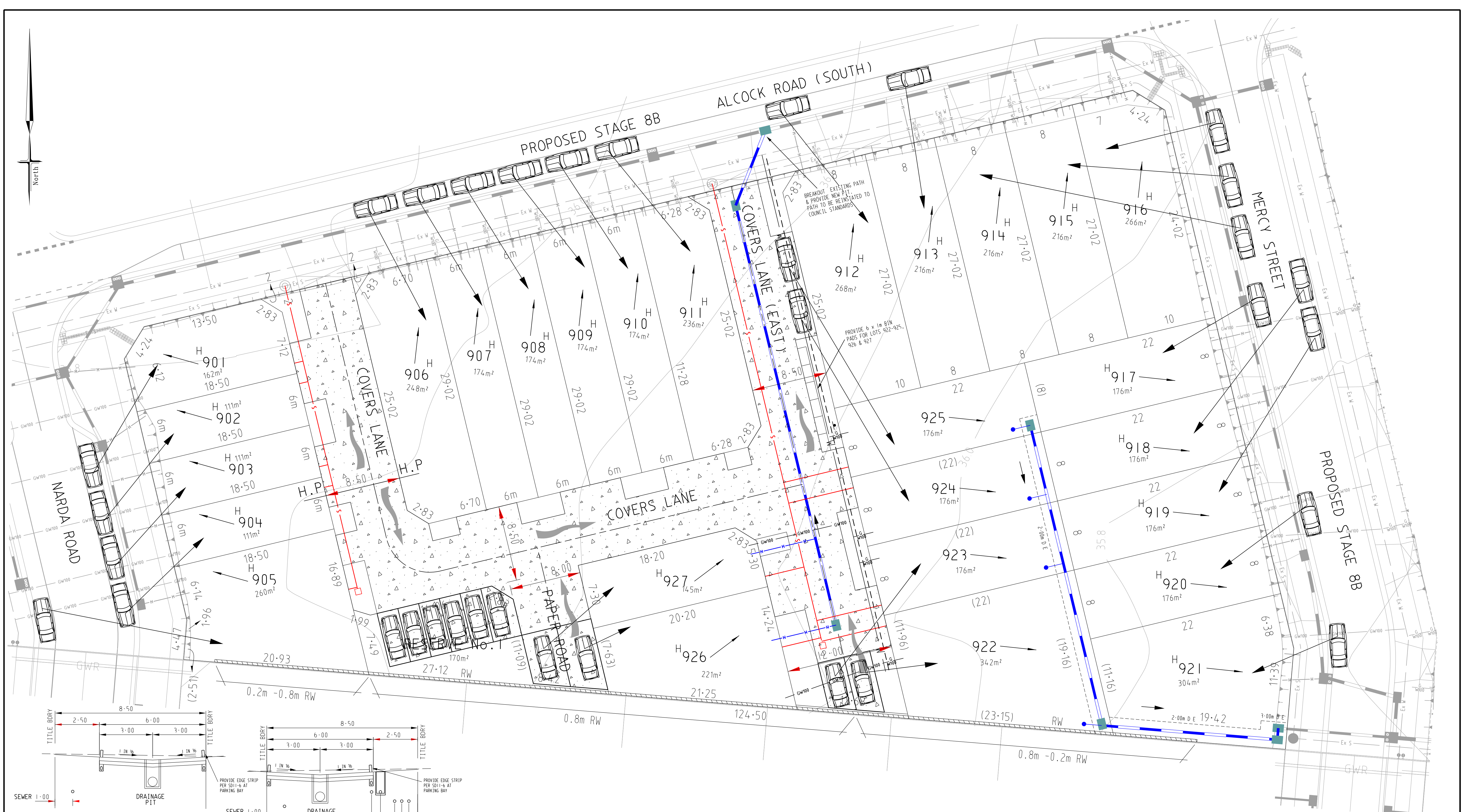
PLAN SCALE 1:200
