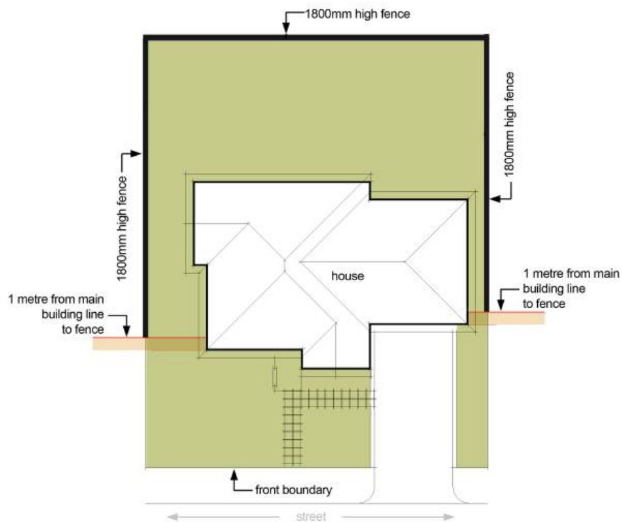
Depiction of typical boundary fencing location
