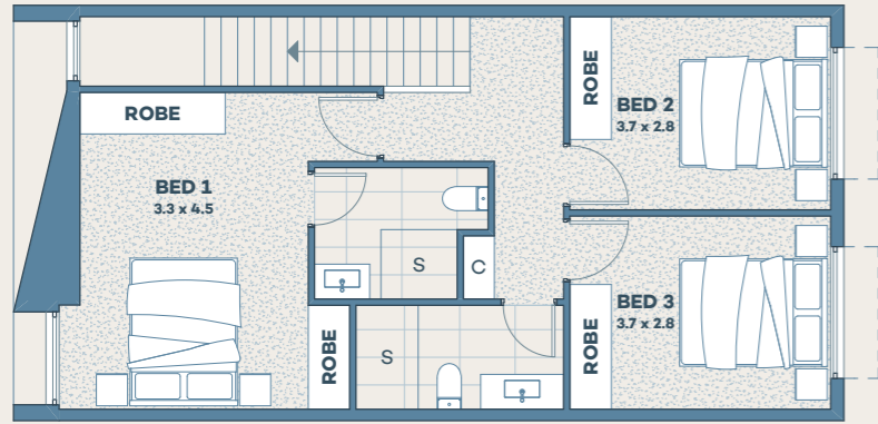
LEVEL 1 PLAN
