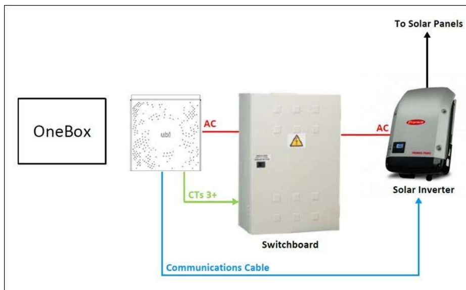
Figure 10: Mondo™Ubi™ connection diagram.
