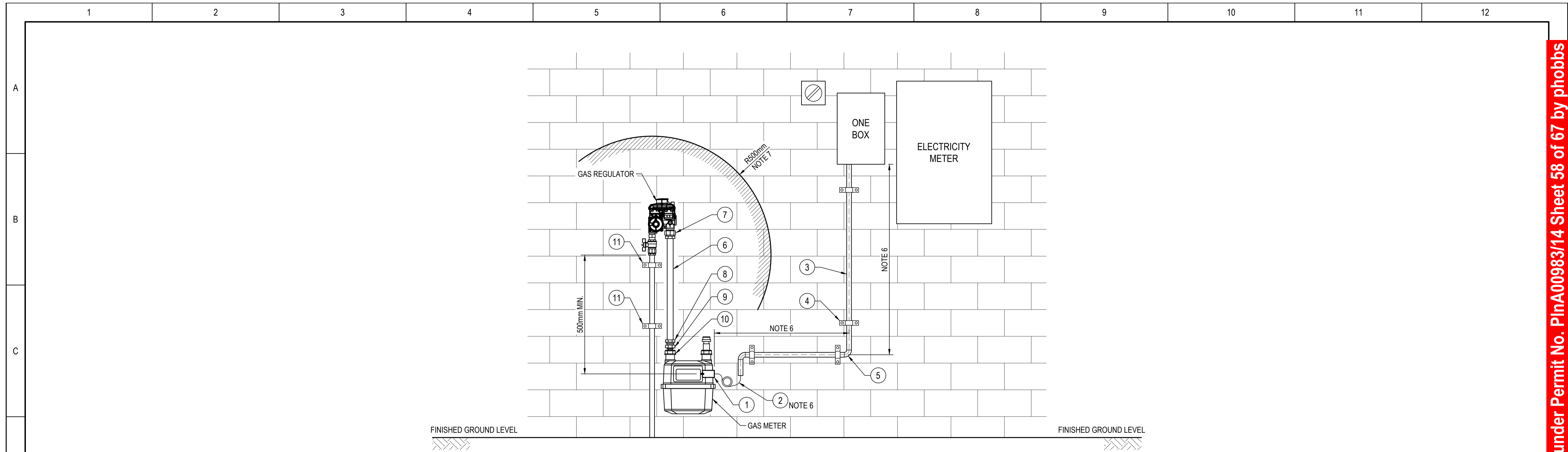
OPTION 2 - VERTICAL SEPARATION OF GAS REGULATOR AND METER NOT TO SCALE
